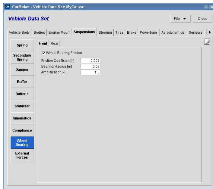
Figure 6.16: Wheel Bearing definition
