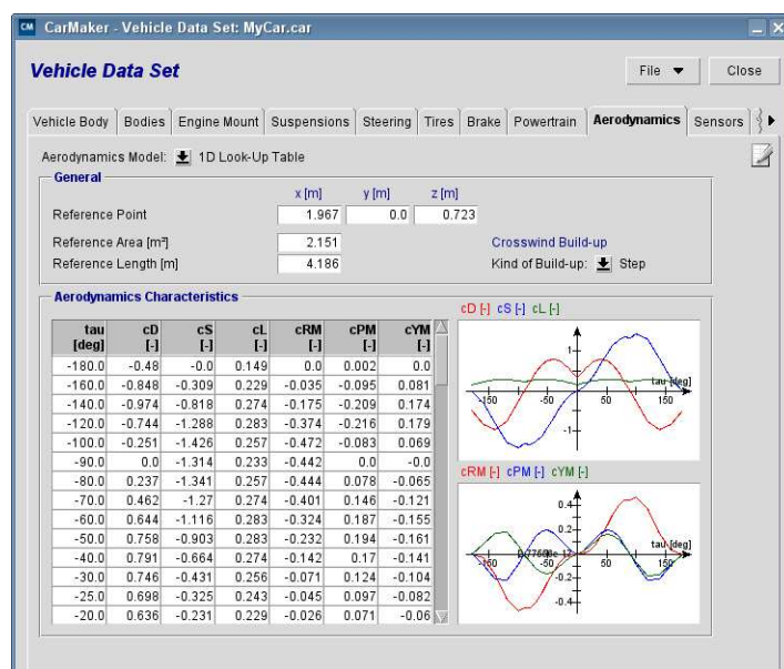
Figure 6.27: Aerodynamics definition
