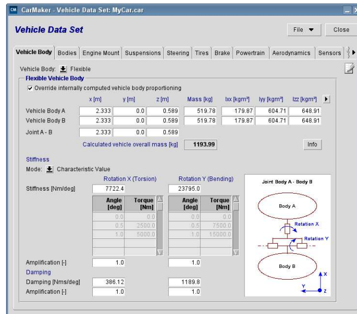
Figure 6.3: Vehicle body
