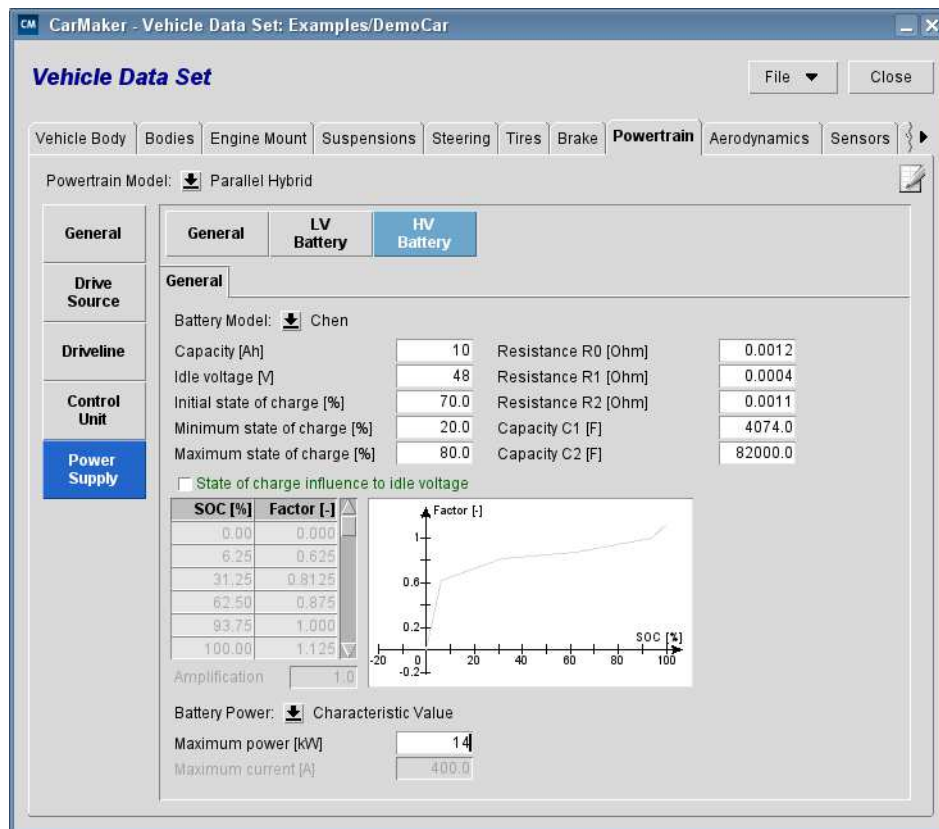
Figure 5.31: Parameterizing the HV Battery
