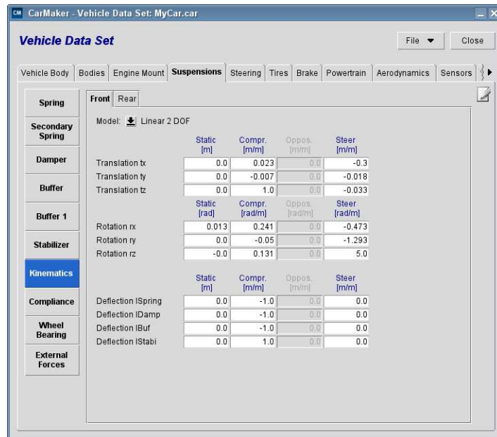
Figure 6.13: Kinematics definition
