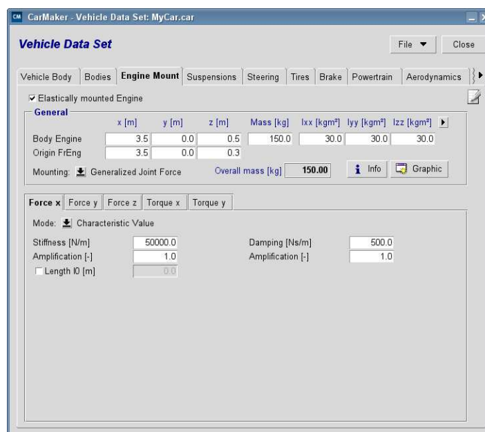
Figure 6.6: Engine definition
