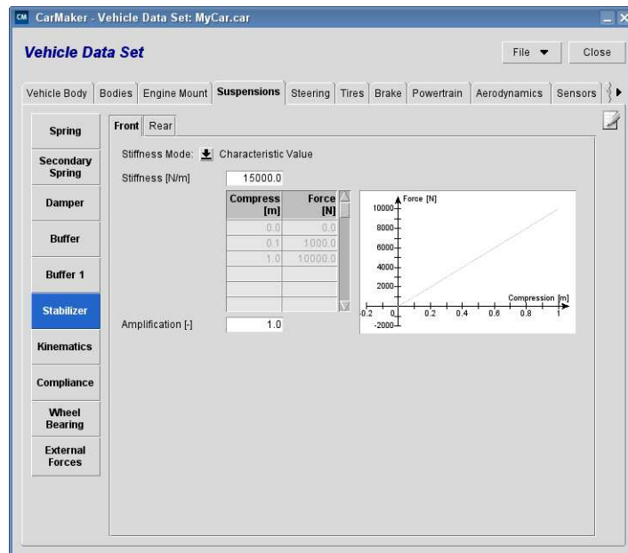
Figure 6.12: Stabilizer definition
