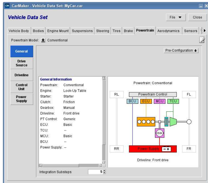
Figure 6.20: Powertrain Model definition
