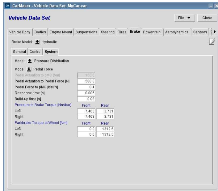
Figure 6.19: Brake system definition
