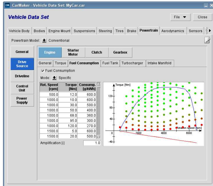
Figure 6.22: Fuel Consumption definition
