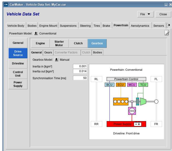
Figure 6.24: Gear box definition
