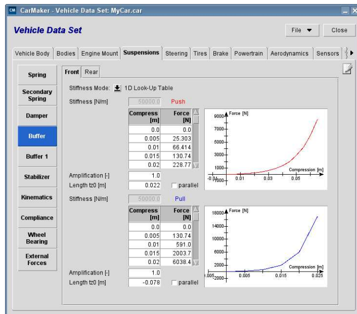
Figure 6.10: Buffer definition
