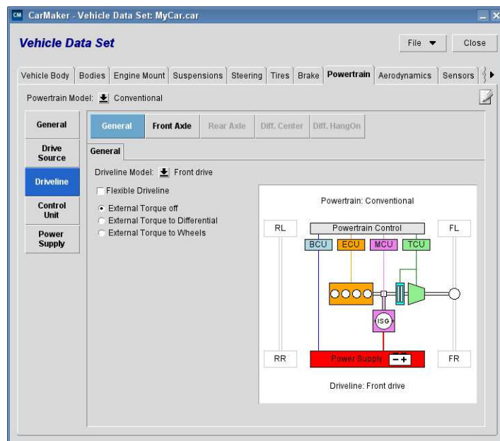
Figure 6.25: Driveline definition
