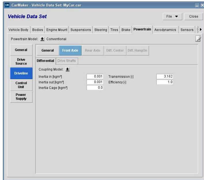
Figure 6.26: Differentials definition
