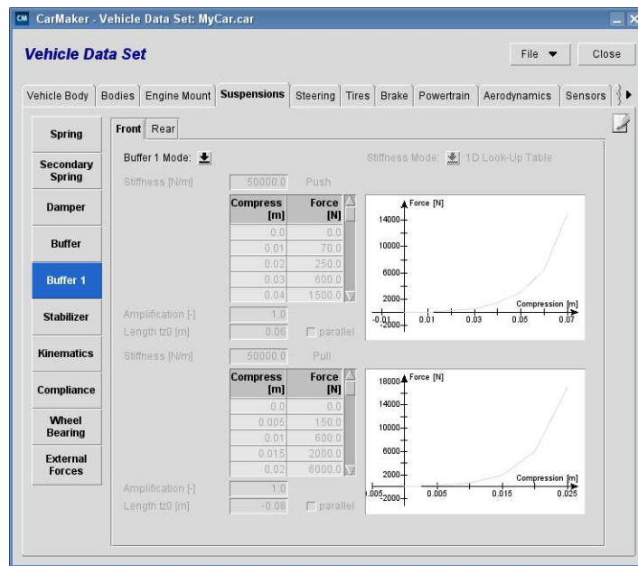
Figure 6.11: Buffer 1 definition
