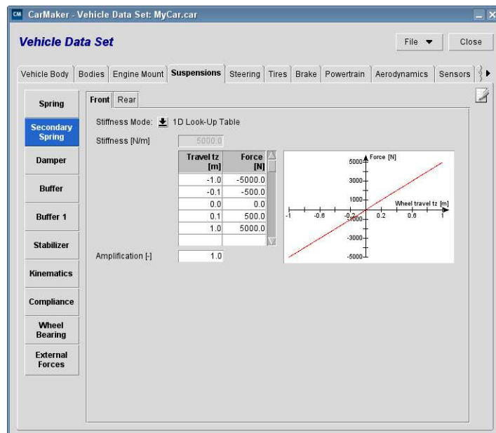
Figure 6.8: Secondary Spring definition
