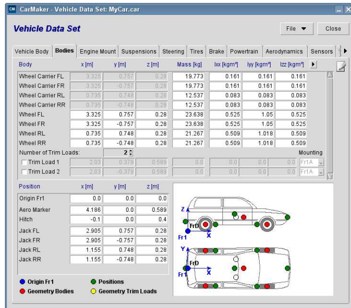
Figure 6.4: Body definition
