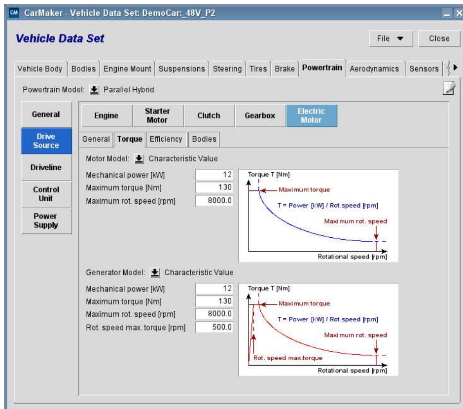
Figure 5.41: Parameterizing the electric motor
