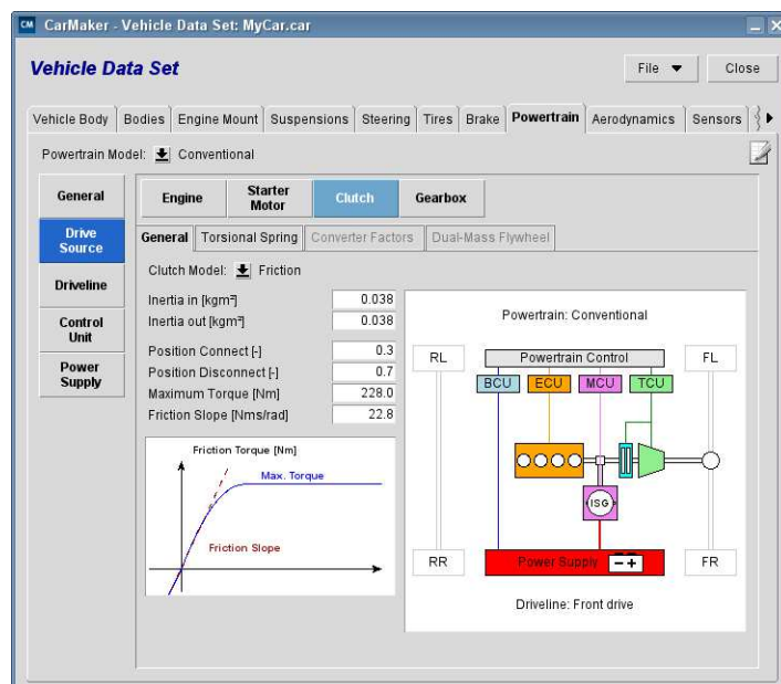
Figure 6.23: Clutch definition
