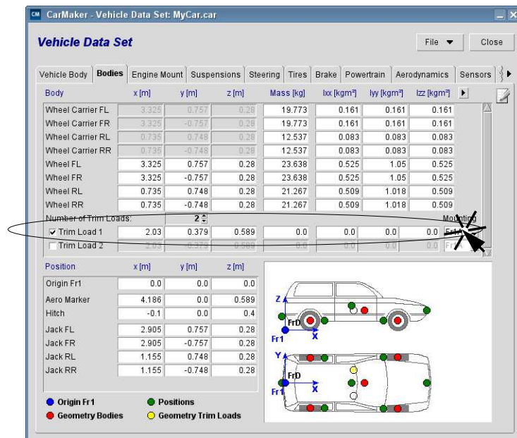
Figure 6.5: Trim Load definition
