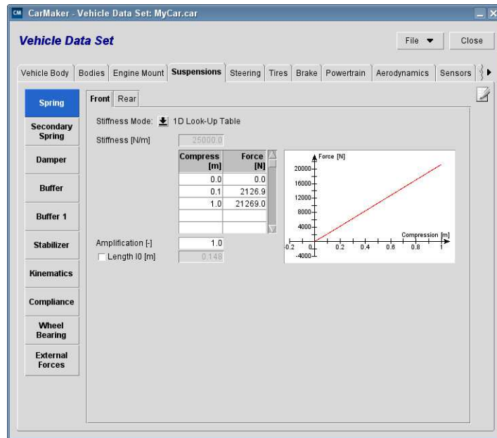
Figure 6.7: Spring definition
