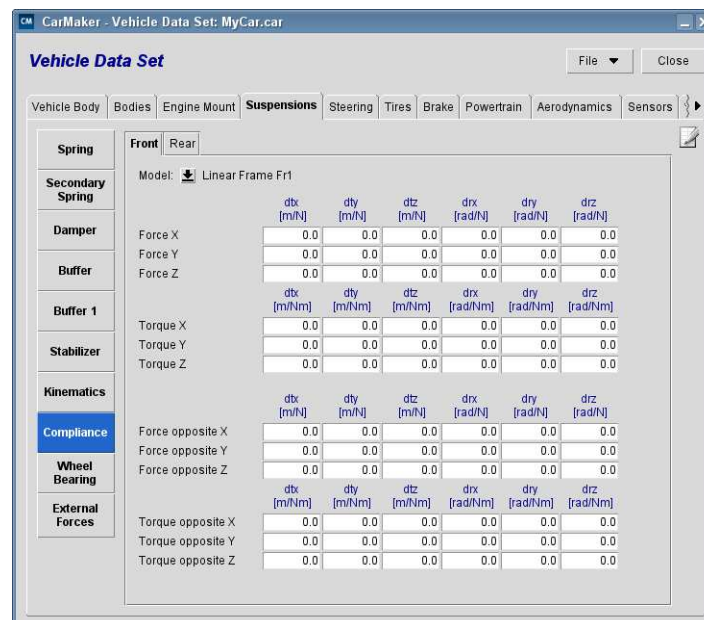
Figure 6.15: Compliance definition
