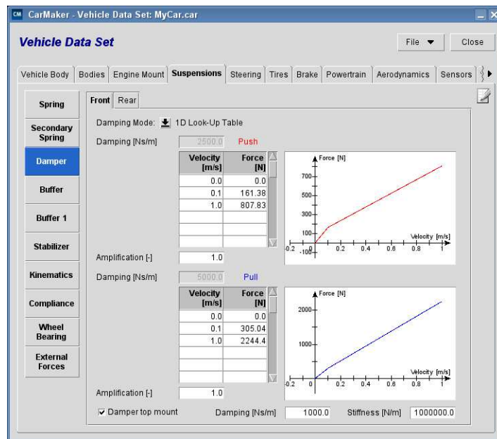
Figure 6.9: Damper definition
